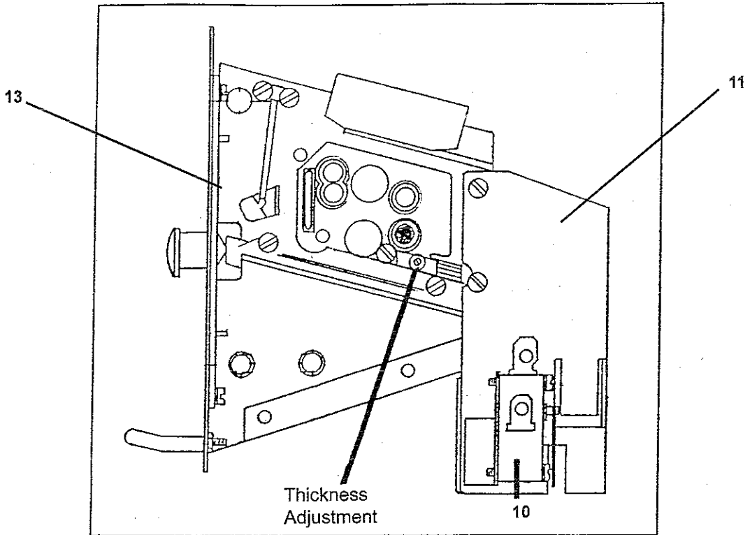
#9 COIN ACCEPTOR - right side
