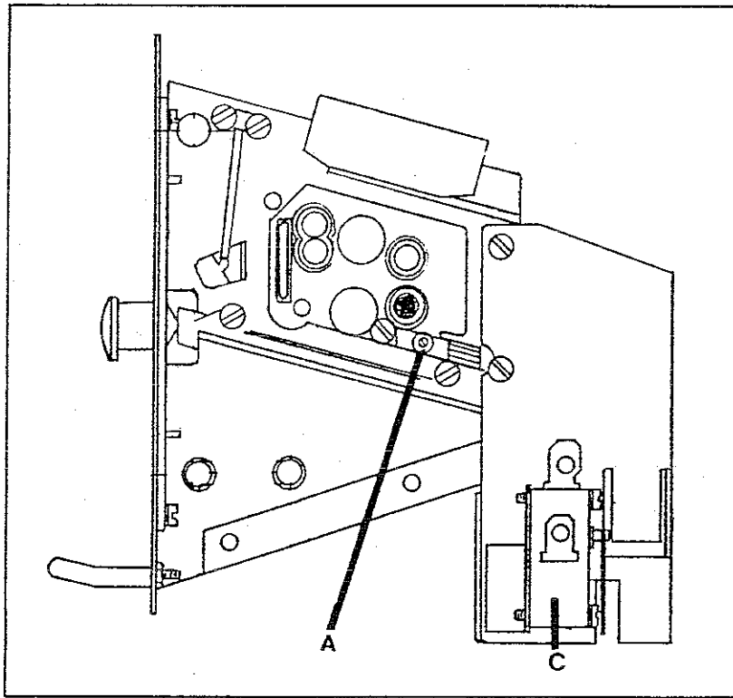
COIN ACCEPTOR - right side
