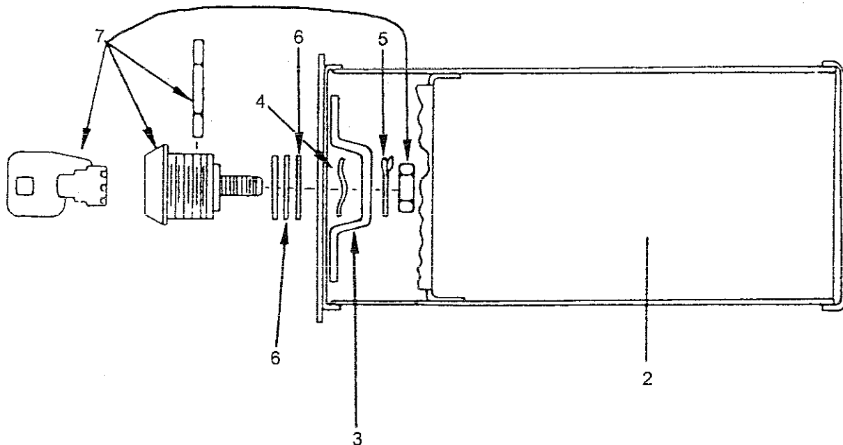
Coin Acceptor From Manual
