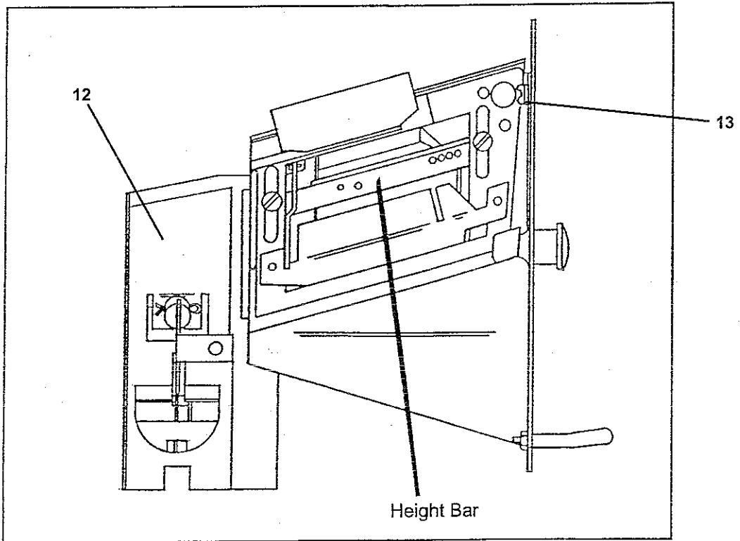
#9 COIN ACCEPTOR - left side
